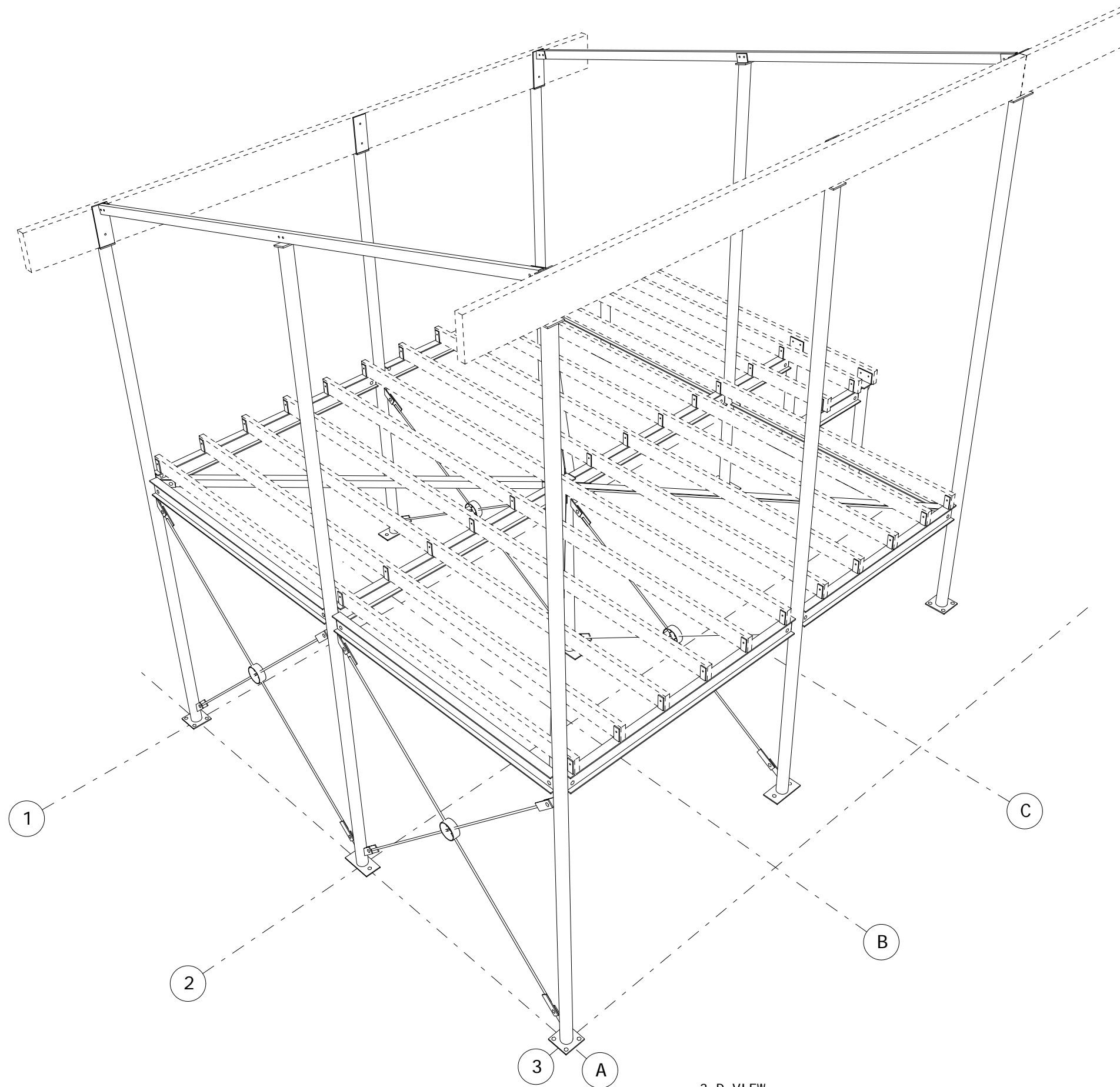
3-D VIEW
